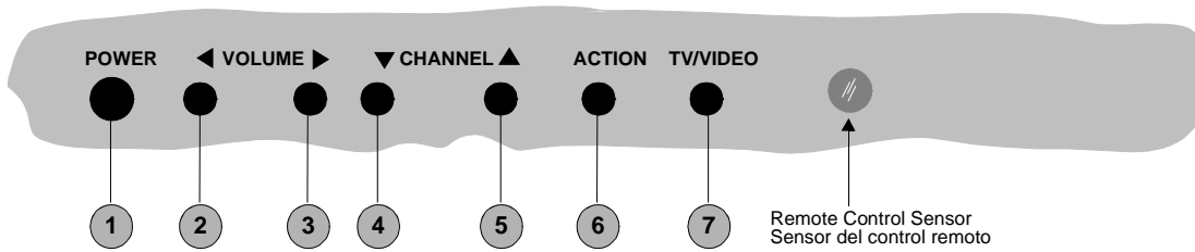
Front Panel for CT-2511H Panel frontal para CT-2511H
